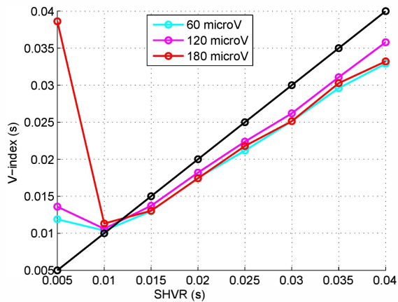
Figure 3. \mathcal{V} -index computed for increasing levels of added noise using three DTW derivatives for the model E.
